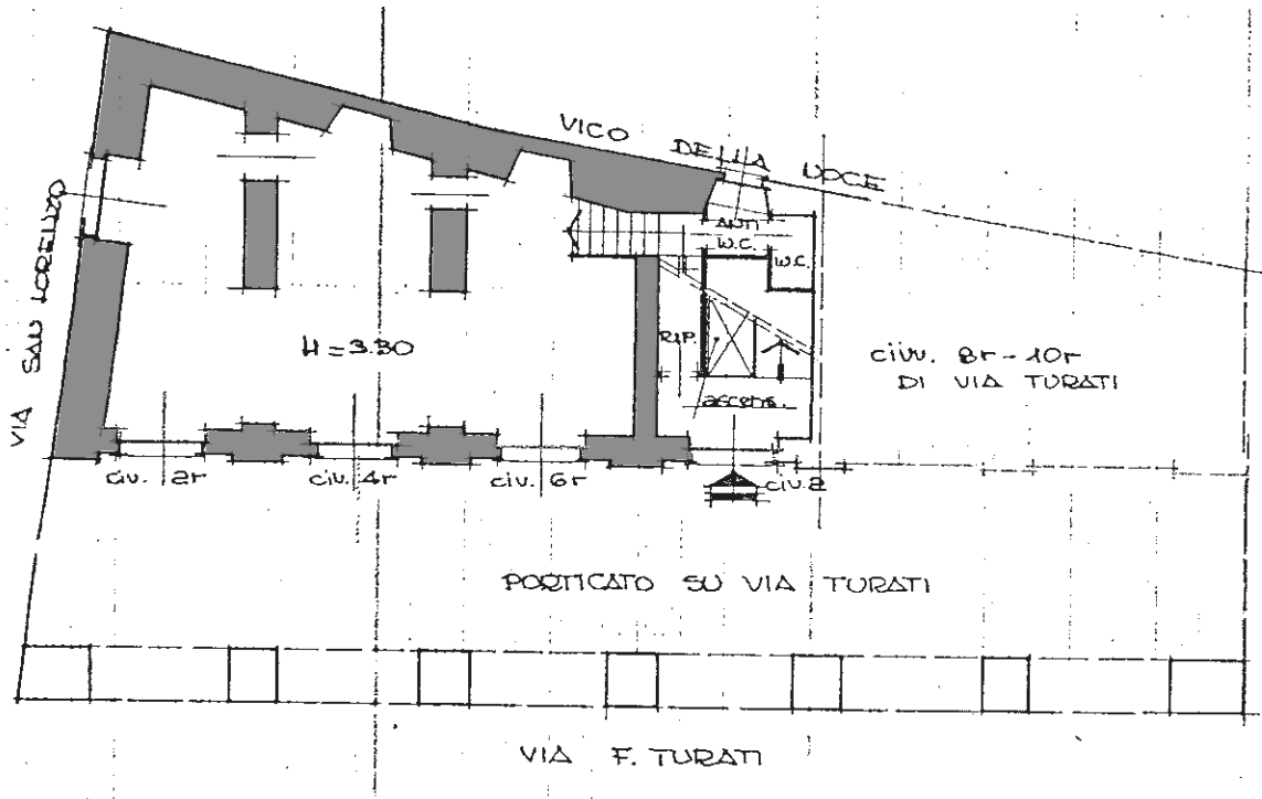
PIANO TERRENO
